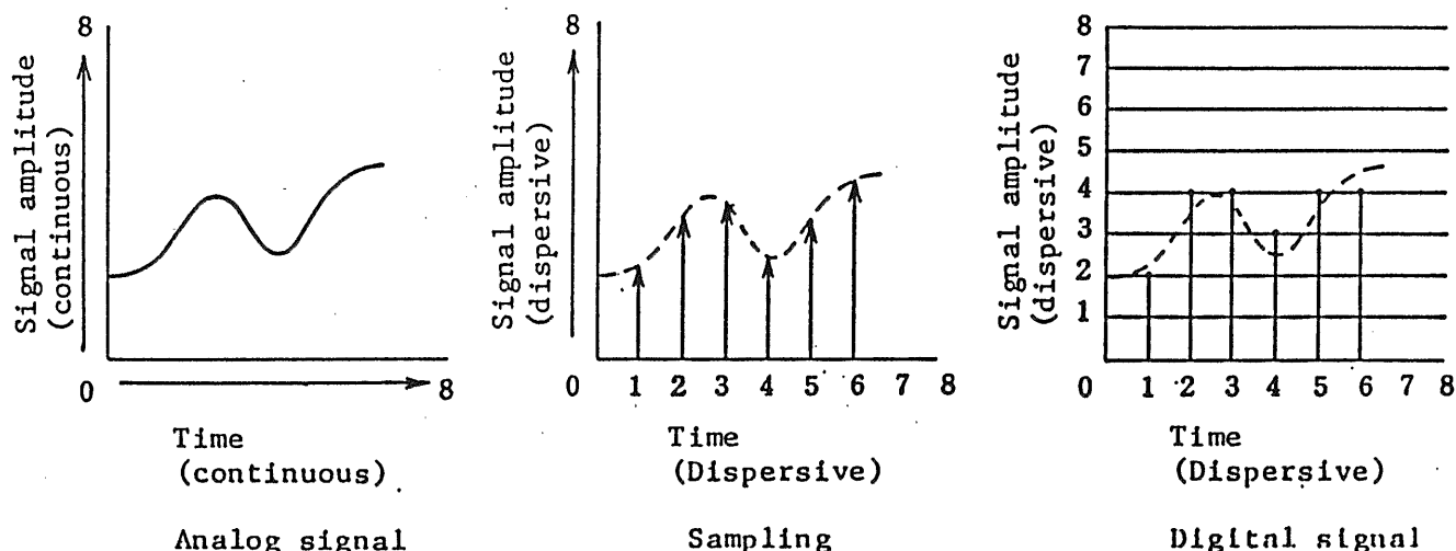
Figure 7-2. A/D Converter
